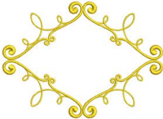
Keystroke A
