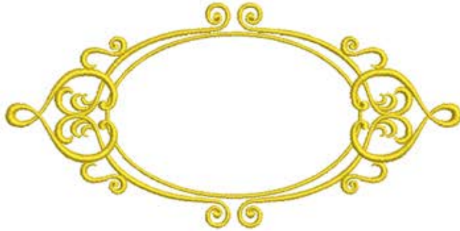
Keystroke C
