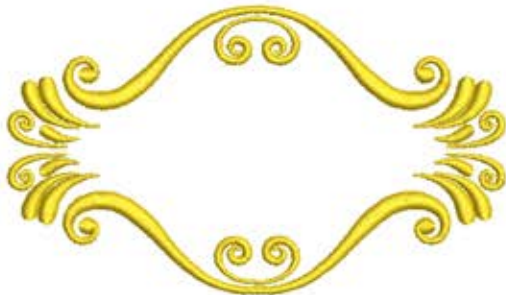
Keystroke E
